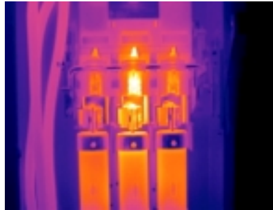
Infrared Image: A Boldstar scan reveals that the switch contacts are heating and require repair. If this condition is not known, electrical fire or power failure will result.
