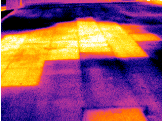
Infrared image, moisture below surface. (bright area)
