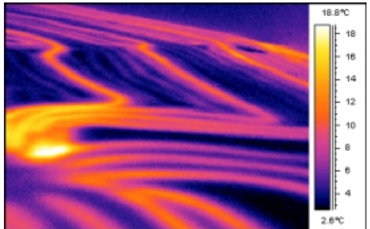
Infrared Image of Underground Parking Ramp Heat Tracing Pipes Sub-Surface Cold Loops and Leaks Located.
