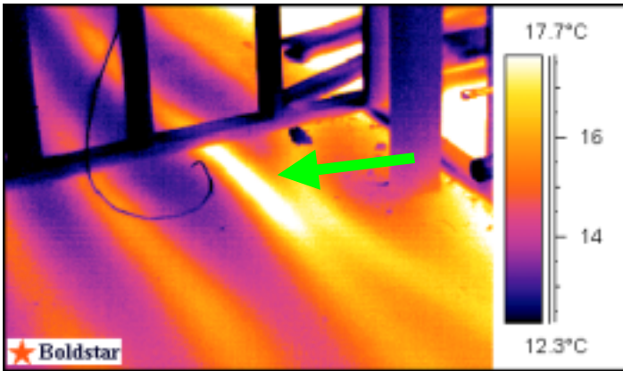
Infrared Image: thermal picture identifies leaks (at arrow)
